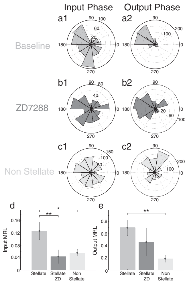
Fig. 6. I_h is necessary for phase specificity of hyperpolarization induced rebound spiking. (a–c) Rose plots for standard inputs in stellate cells ( n = 6 ) before (a) and after (b) application of ZD7288 as well as in non-stellate cells ( n = 7 , c). Rose plots display phase histograms for hyperpolarizing input pulses that induce spiking (a1, b1, c1) and for output spiking phase (a2, b2, c2). (d) Summary bar graph demonstrates that following h -current blockade, stellate cells lose the phase specificity for hyperpolarizing input, as indicated by a significant decrease in hyperpolarizing input MRL (paired t -test, **p < 0.01 ). Furthermore, this significant lack of input specificity is also present in non-stellate cells compared to baseline stellate cells (paired t -test, *p < 0.05 ). (e) Summary bar graph demonstrates that blocking the h -current in stellate cells decreases the specificity of output spiking phase, shown by a decrease in the MRL of output spiking phase, but this does not reach statistical significance. However compared to stellate cells, non-stellate cells display a significantly smaller MRL (paired t -test, **p < 0.01 ), and therefore, less phase specificity of output spiking.
